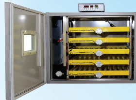
NH-264 Capacity:264eggs Size:740*600*1090mm Weight:46kg
