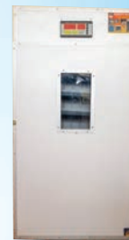
NH-528 Capacity:528eggs Size:1050*630*1260mm Weight:68kg
